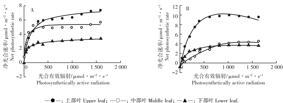
图1 蕾后期和花前期切花菊品种‘神马’不同部位叶片的光响应曲线 Fig. 1 Light response curve of leaves in different positions of cultivar ‘Jinba’ of cut chrysanthemum ( Chrysanthemum morifolium Ramat.) at post-budding and pre-blooming stages
